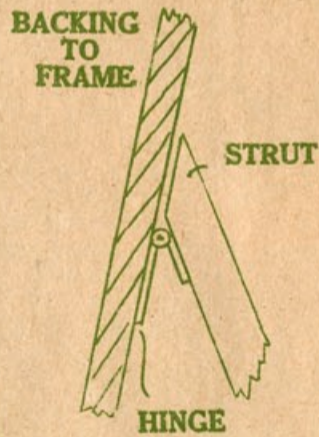
DETAIL OF HINGE & STRUT.
