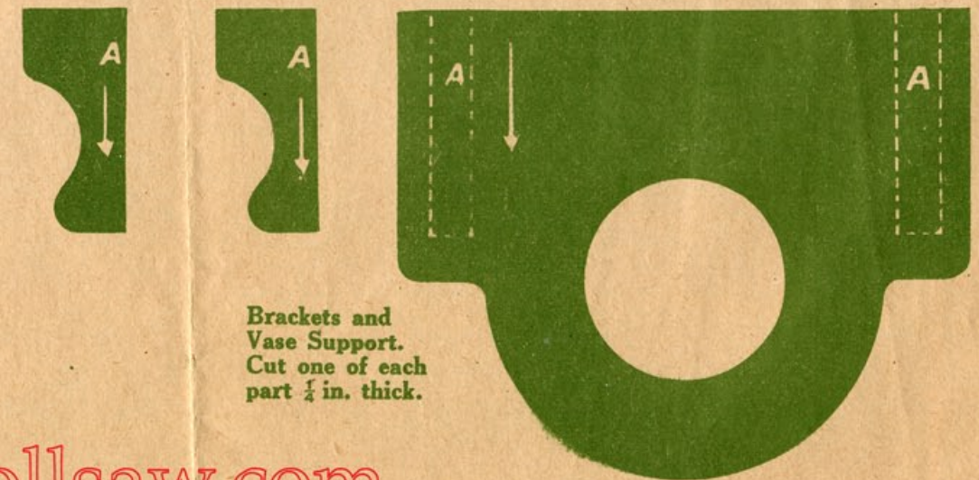
Brackets. Cut one of each 1/4 in. thick.
