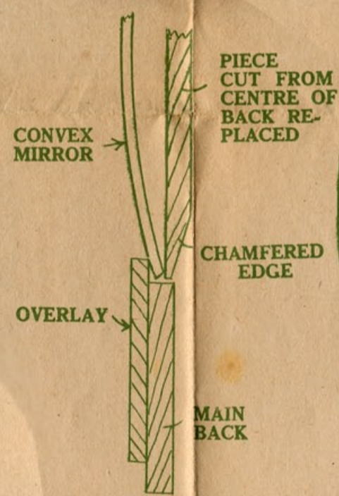
SECTION THROUGH MIRROR & OVERLAY
