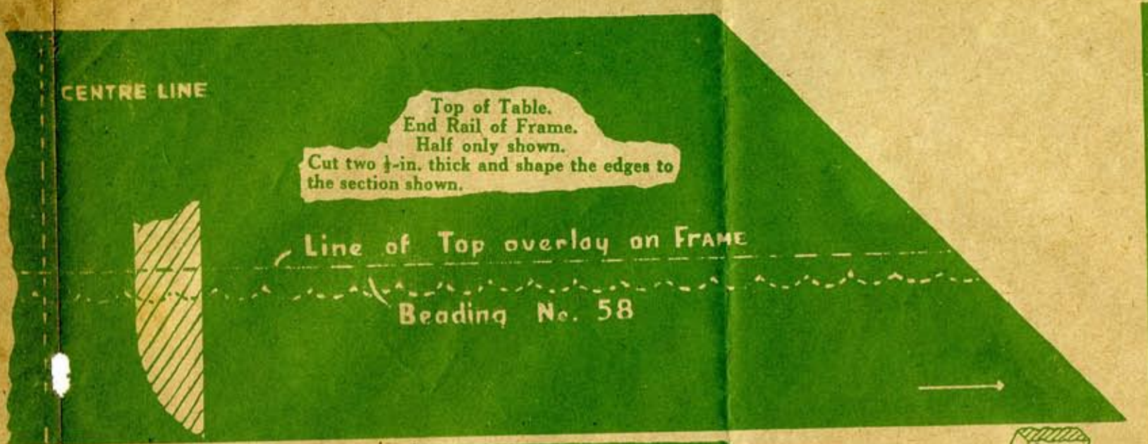
Detail showing how tops of Legs are cut to receive ends of Rails.
