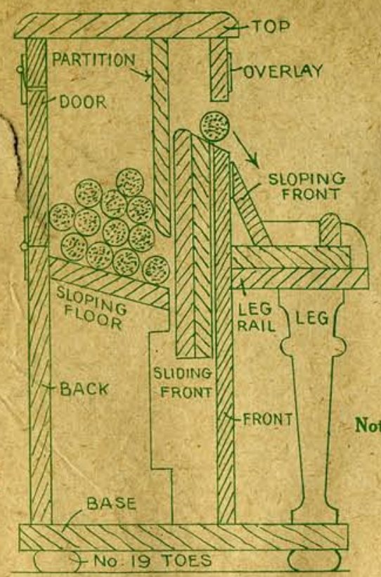
SECTION SHOWING POSITIONS OF THE VARIOUS PARTS AND THE SLIDING FRONT RAISED. DETAIL NOT FULL SIZE.
